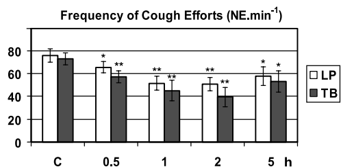
Fig. 2. Frequency of cough efforts (NE.min -1 ) after the administration of 200 \text{ mg}\cdot\text{kg}^{-1} b.w. of EEPF p.o. For explanation see Fig. 1.
